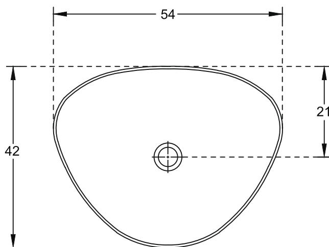
PLAN VIEW
