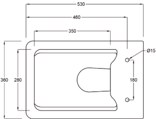
PLAIN-VIEW
