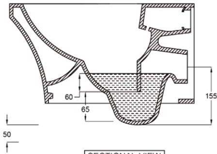
SECTIONAL-VIEW
