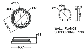
CARTRIDGE LOCK NUT
